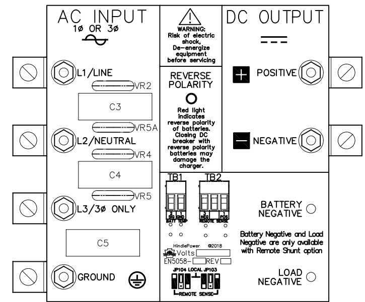
ST-5070 I/O TERMINAL BOARD DETAIL
