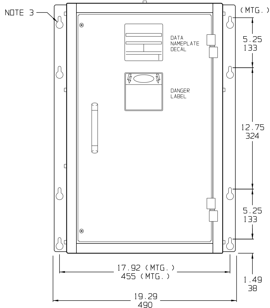
FRONT VIEW
