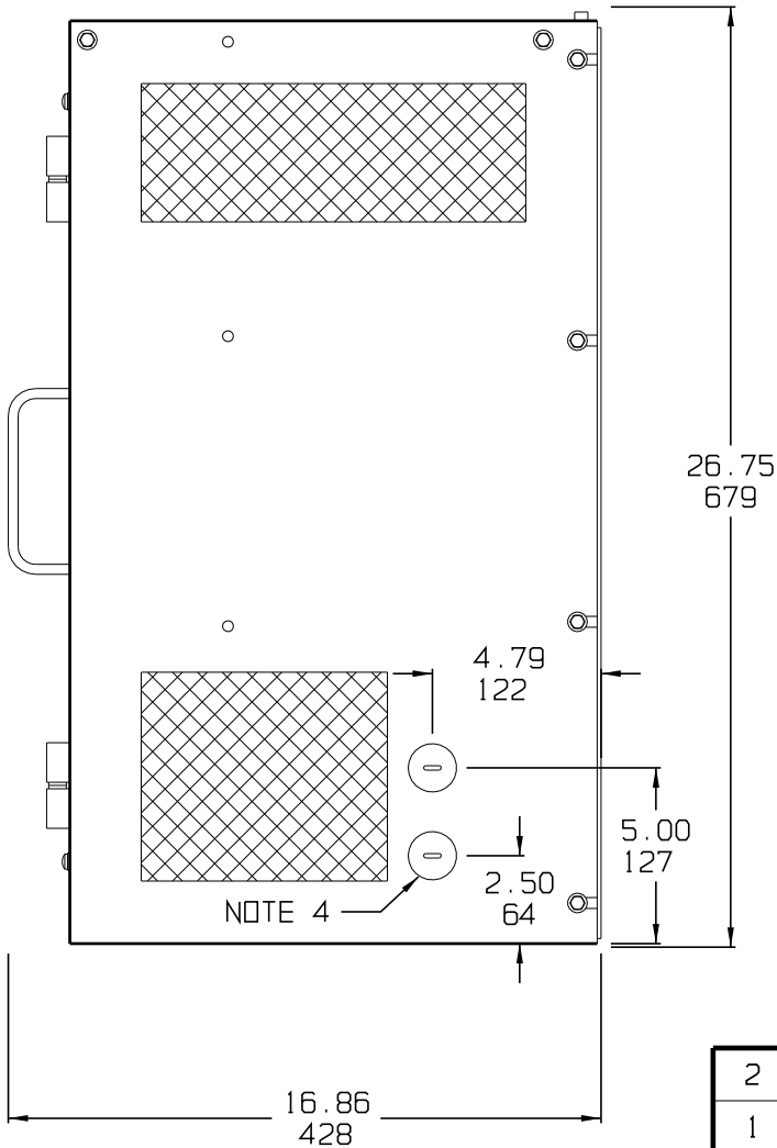
SIDE VIEW
